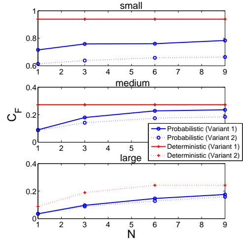
Fig. 4. Forbidden area coverage versus number of UAVs
