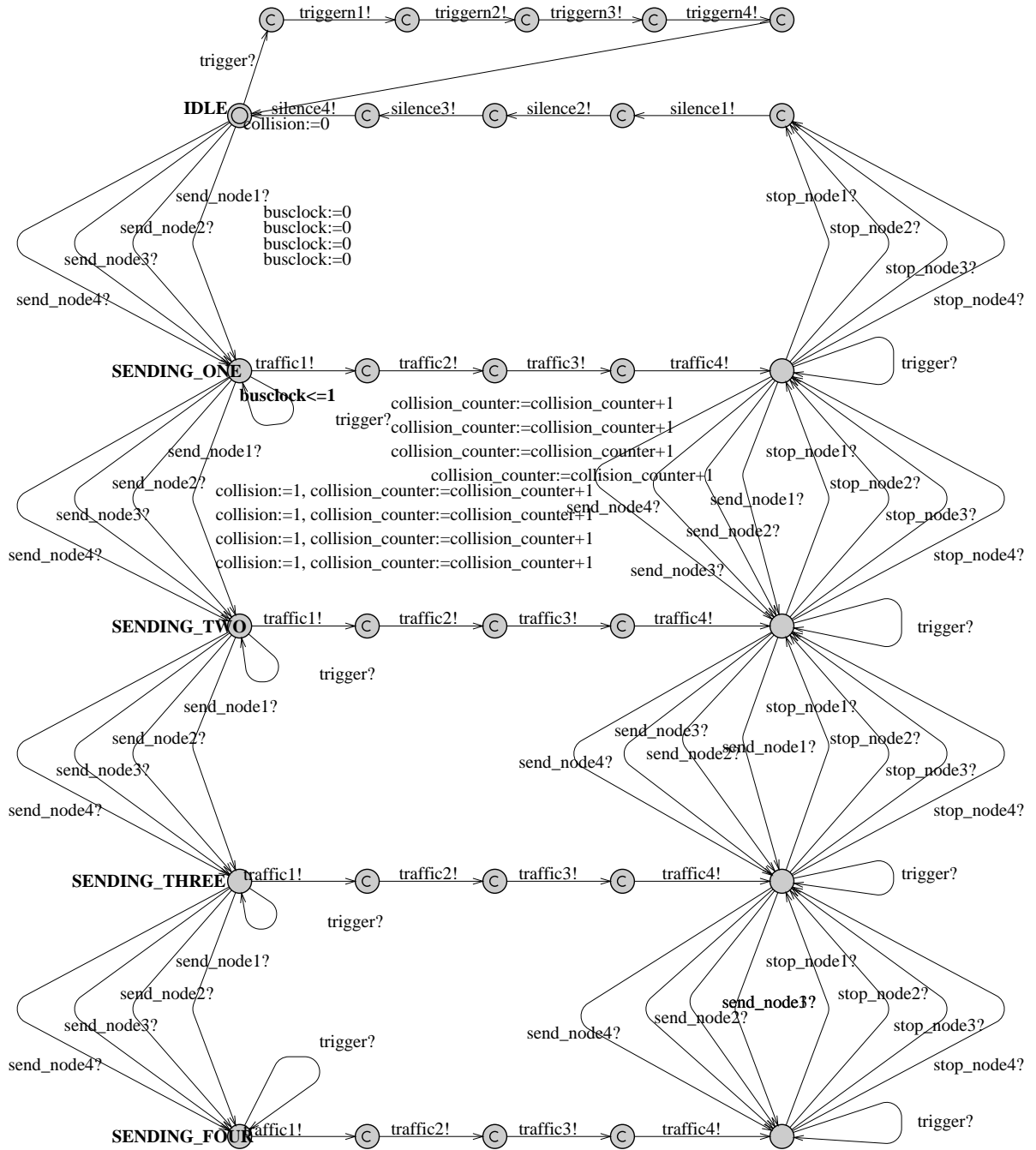
Figure 9: Model of TTP/A channel
